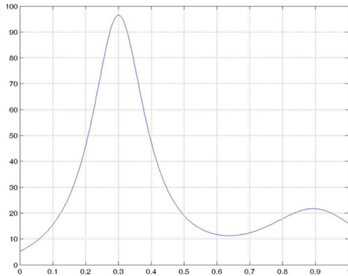
Figure 1: Function humps(x)
