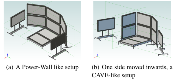
Figure 7: The Concept shown in Sketches
