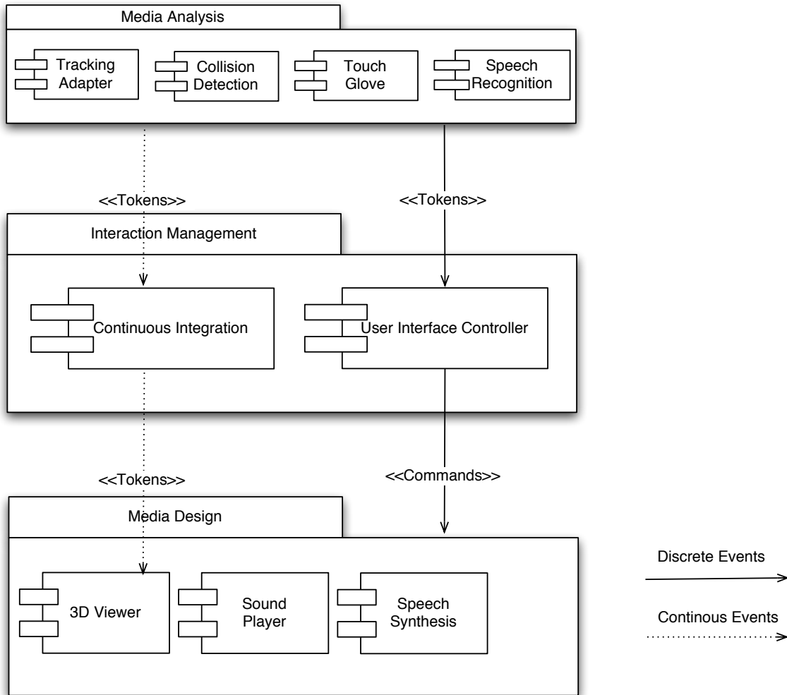
Figure 2. Functional decomposition of DWARF specific user interface components
