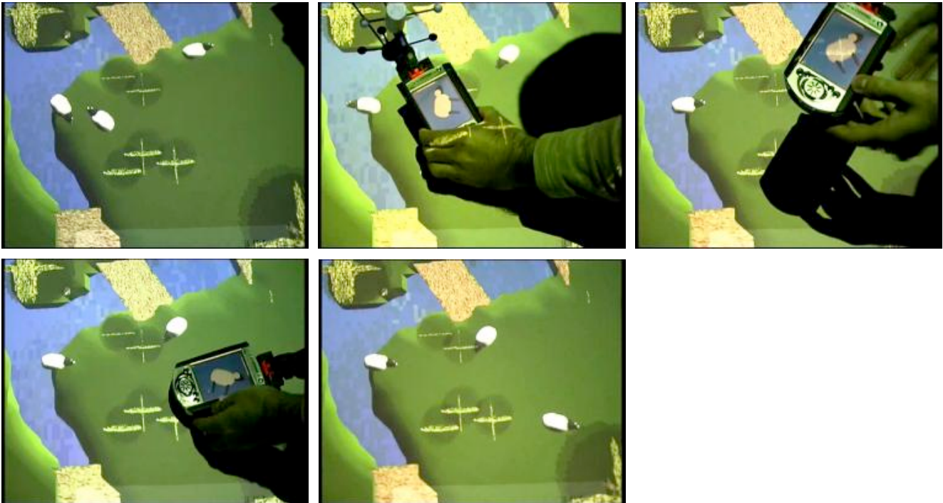
Figure 10. Scooping a virtual sheep with an iPAQ that acts as tangible display
