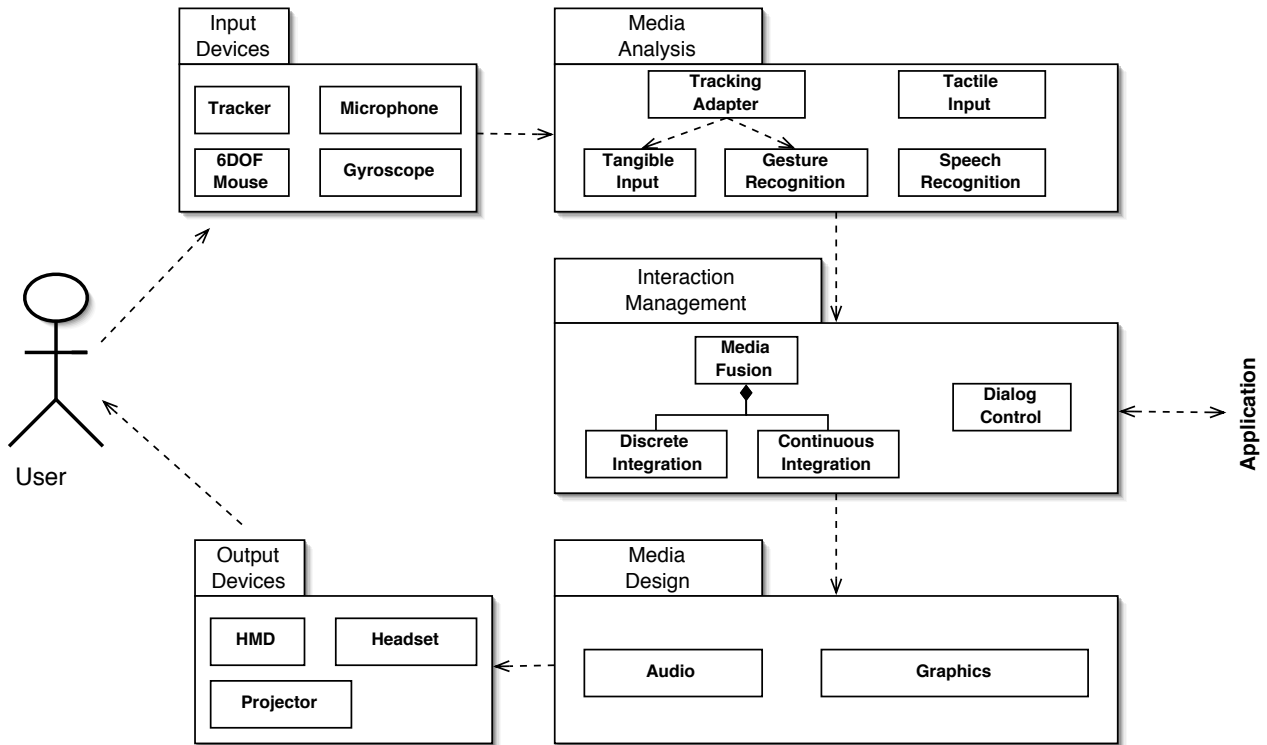
Figure 1. A generic functional decomposition of Ubiquitous Augmented Reality User Interfaces
