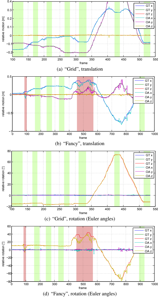
Figure 5: Motion curves for marker tracker (ground truth, “GT”) and our approach (“OA”) for the basic “Grid” design (a),(c) and the basic “Fancy” design (b),(d) test cases. Diagrams (a) and (b) plot the relative movement of the object’s center over time. Diagrams (c) and (d) show rotational movement along the object’s coordinate axes. The offset between car origin and marker board origin is already compensated. Note that the object was moved along the primary plane of the marker board only so that translation along Z and rotation around X and Y were almost constant. Green areas mark frames where the object was not moved. This data is evaluated separately in Table 1 (“Rest”). Clearly visible is the response time of our method after translational movement (for instance in diagram (a), frame 140-160 and 190-210). The ICP algorithm temporally diverged for the “Fancy” test case (red areas).
