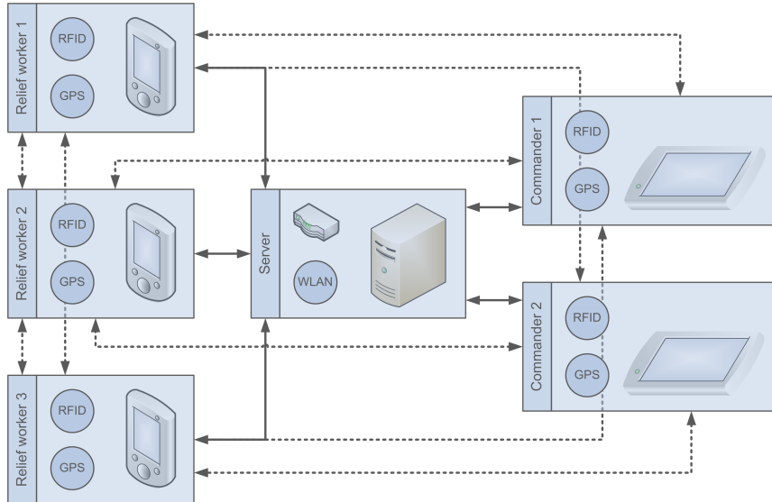
Figure 1: System Architecture
