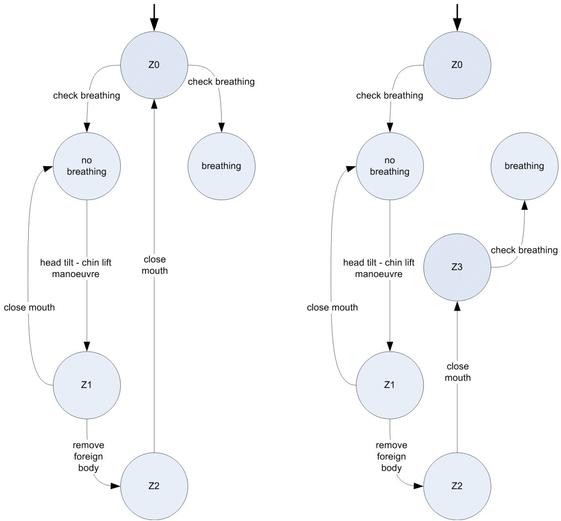
Figure 4: State automaton. (a) The general non-deterministic finite state automaton (b) The patient specific deterministic finite state automaton
