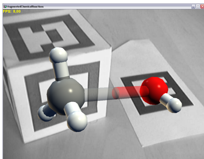
(a) One possible bond between two atoms
