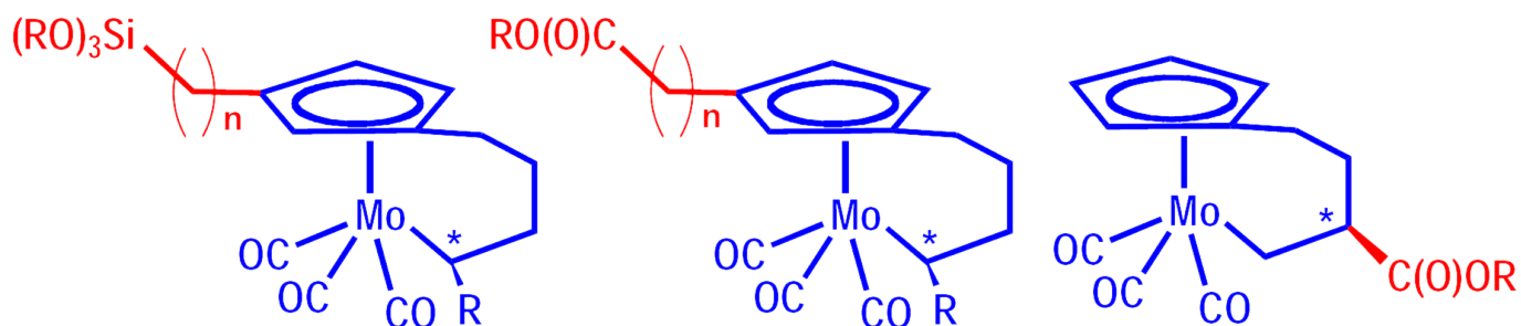
Fig. 7. Organomolybdenum complexes
