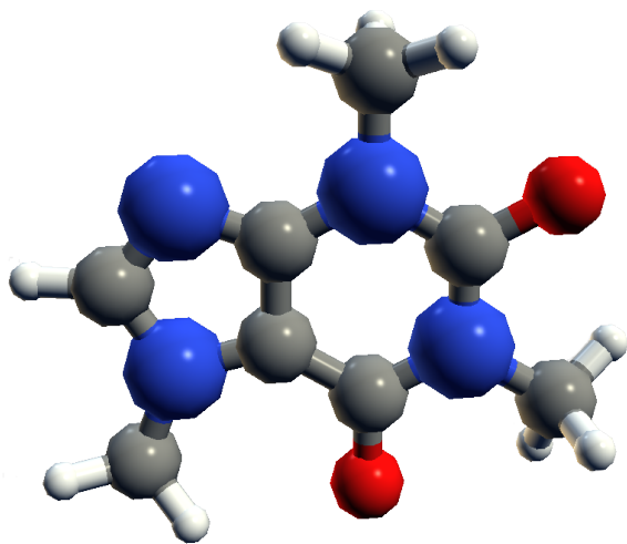
Fig. 1. Ball and Stick Model
