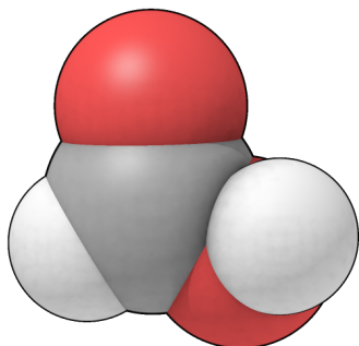
Fig. 2. Space Filling Model
