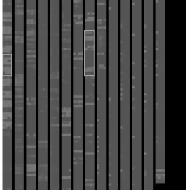
Figure 4: Overview window.
