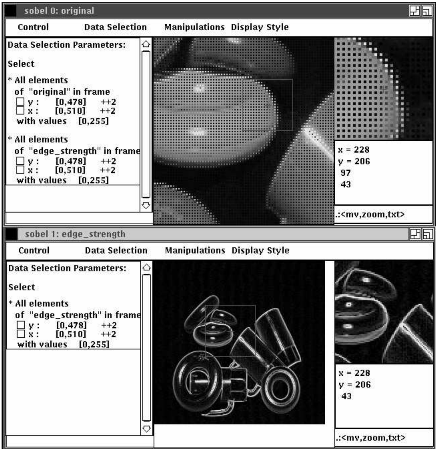
Figure 2- 7 Links between arrays
