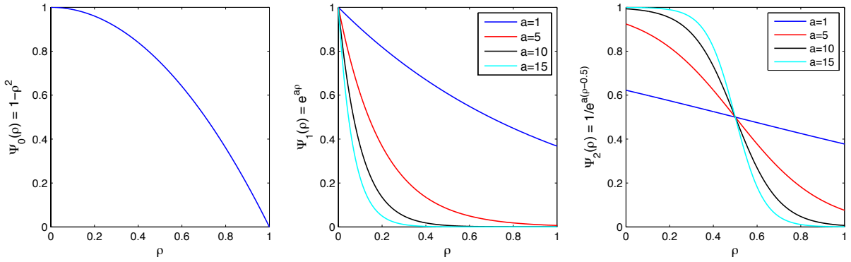
Fig. 4. Three types of weighting functions considered for our proposed method. (a) \Psi_0(\rho) = 1 - \rho^2 , (b) \Psi_1(\rho) = e^{-a\rho} , and (c) \Psi_2(\rho) = \frac{1}{1 + e^{a(\rho - \frac{1}{2})}} .
