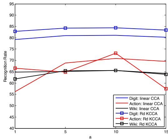
Fig. 13. Comparisons of recognition rates using different a for each dataset. Note that Action, Digit, and Wiki stand for IXMAS Multi-View, UCI Multiple-Features, and Wikipedia datasets.
