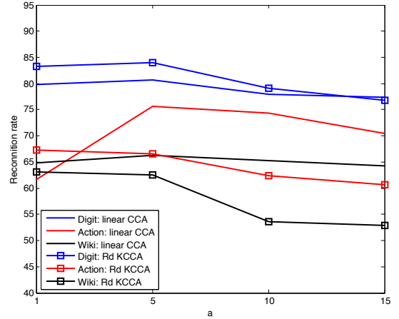
Fig. 12. Comparisons of recognition rates using different a for each dataset. Note that Action, Digit, and Wiki stand for IXMAS Multi-View, UCI Multiple-Features, and Wikipedia datasets.
