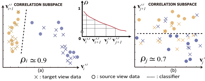
Fig. 3. Projecting source and target view instances from the IXMAS dataset into different correlation subspaces using CCA projection vectors with different \rho .
