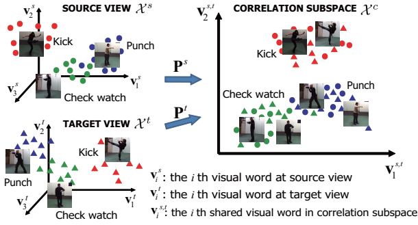
Fig. 2. Domain adaptation via CCA [2]. Note that \mathbf{P}^s and \mathbf{P}^t are the projection matrices produced by CCA, which maximize the correlation between projected data in the derived subspace \mathcal{X}^c
