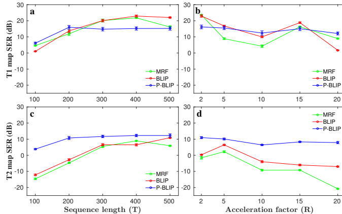
Fig. 3. a,c , Performance as a function of sequence length with R = 10 , P = 3 \times 3 ; and b,d , as a function of acceleration factor with T = 200 , P = 3 \times 3 . P-BLIP is best in estimating T2 maps and shows better results for shorter sequences and higher acceleration for T1 maps.
