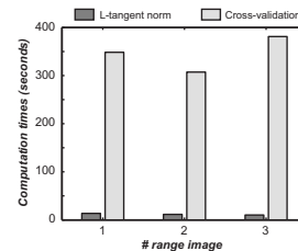
Figure 10. Computation time needed to reconstruct the whole surface from the range images of figures 6a and figure 7 using the L-tangent norm and cross-validation.
