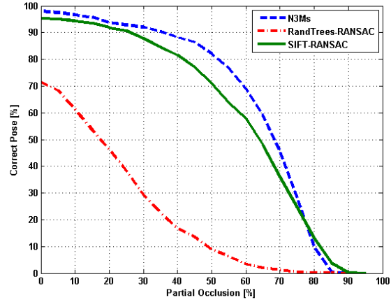
Figure 6. Natural 3D Markers versus Randomized Trees and SIFT
