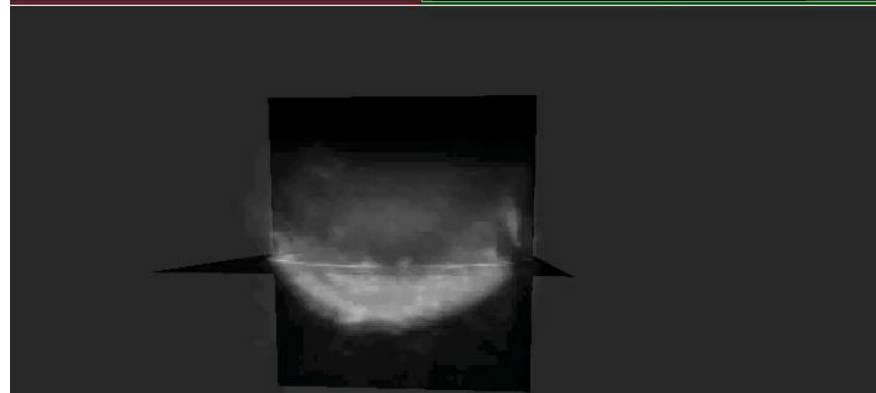
SLAM
